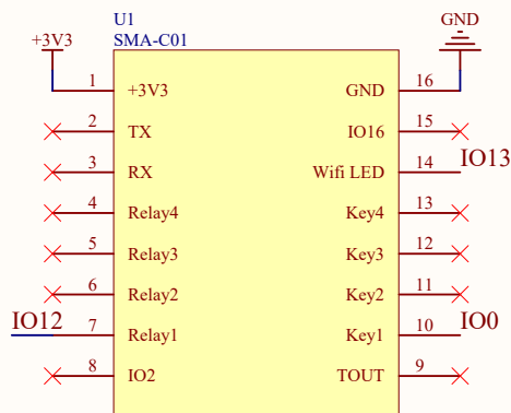
SMA-C01模块
